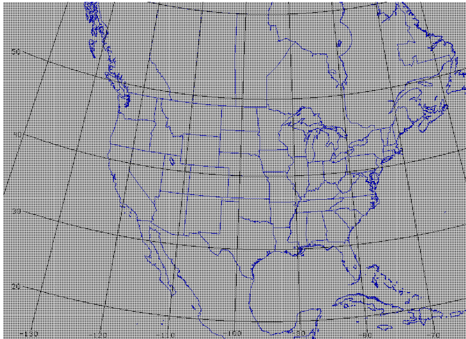
Figure 2.3. UCAR-NAM-CONUS-12km domain.
